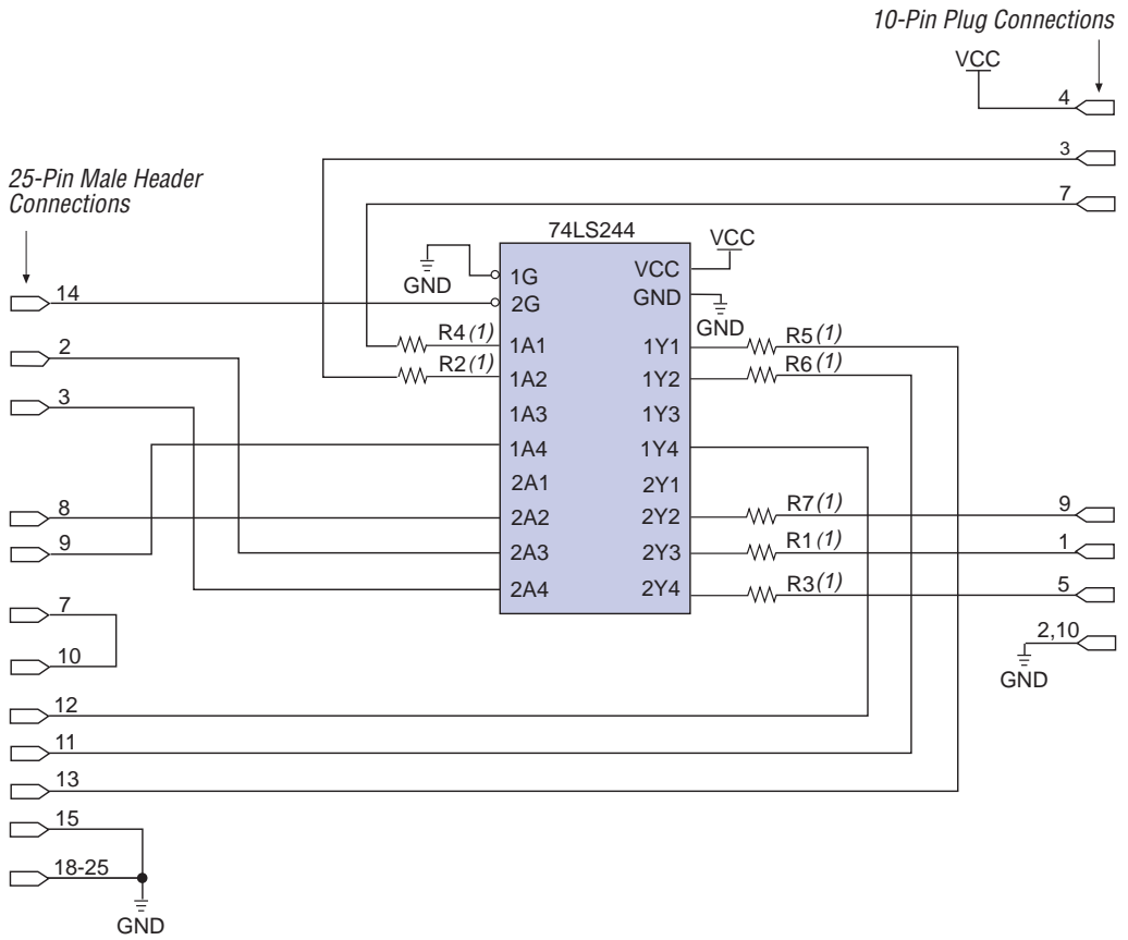
Figure 2. ByteBlaster Schematic
